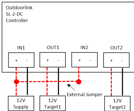
Single Supply w/ 2 Target Devices
