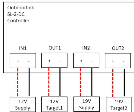
Dual Supply w/ 2 Target Devices
